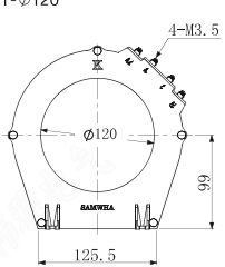
ZCT-Ø120
