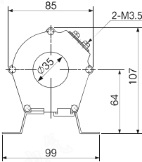
ZCT-Ø35
