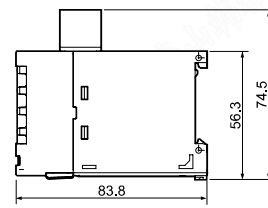
PANEL&DINRAILTYPE
