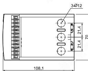
PANEL&DINRAILTYPE
