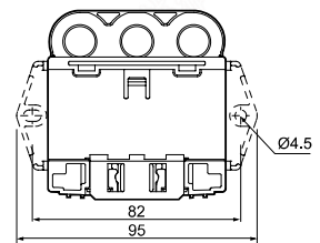
MOUNTINGHOLESIZE
