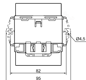
MOUNTINGHOLESIZE
