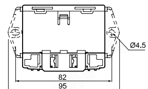
MOUNTINGHOLESIZE
