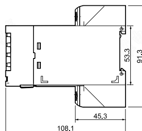
PANEL&DINRAILTYPE
