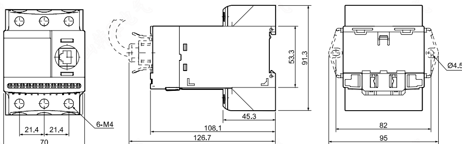
PANEL&amp;DINRAILTYPE
