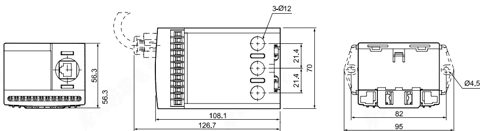
PANEL&amp;DINRAILTYPE
